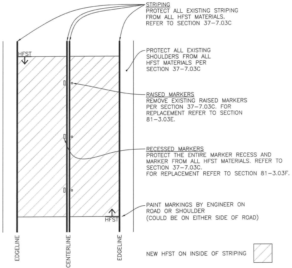
TYPICAL HFST INSTALLATION PLAN NTS
