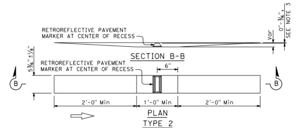
RECESS DETAIL FOR RETROREFLECTIVE PAVEMENT MARKER
