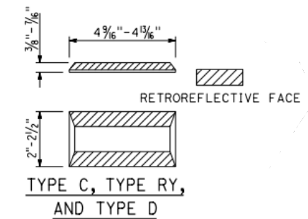
RETROREFLECTIVE PAVEMENT MARKER FOR RECESSED INSTALLATION See Notes 1 and 2
