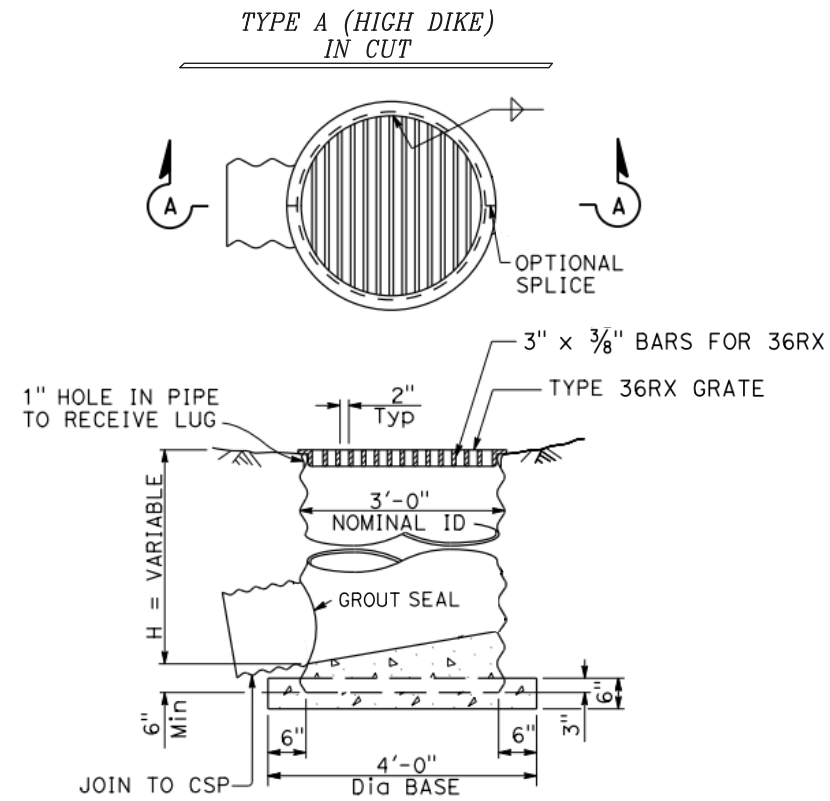
SECTION A-A TYPE GMP Steel pipe inlet with grate
