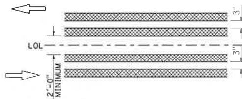
DETAIL 28
