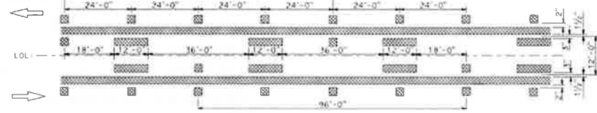
DETAIL 32
