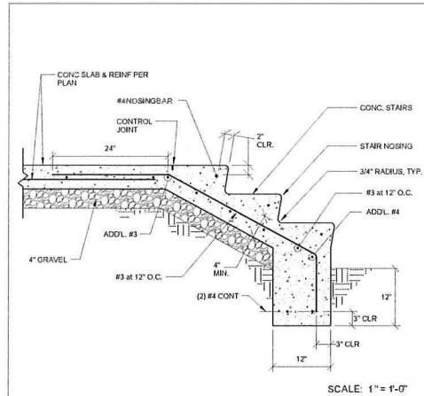
EXTR CONC. STAIR ON GROUND DET 405
