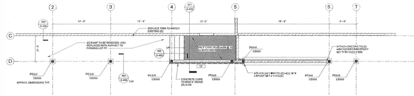
FOUNDATION PLAN 1/4" = 1'-0"
