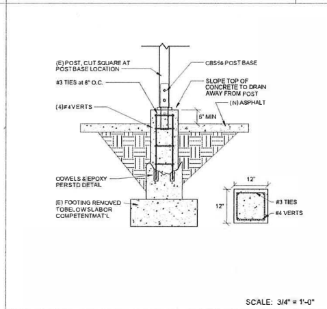
PIER FOOTING DETAIL 404
