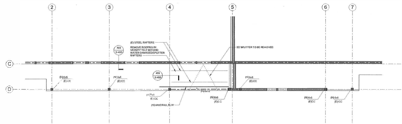
FRAMING PLAN 1/4" = 1'-0"
