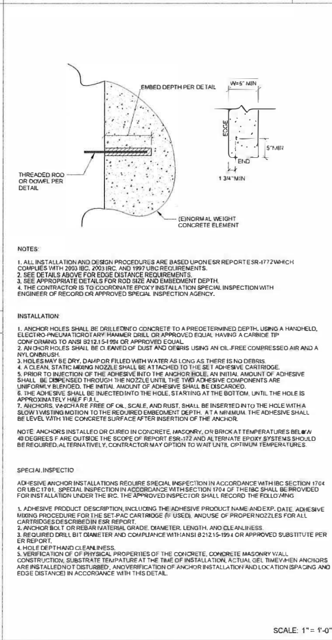
TYP EPOXY INSTALLATION PROCEDURE 401
