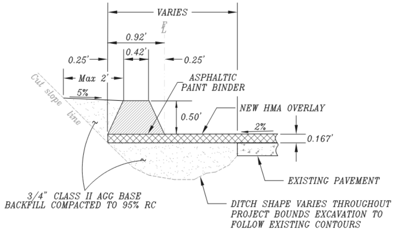
TYPE A (HIGH DIKE) IN CUT
