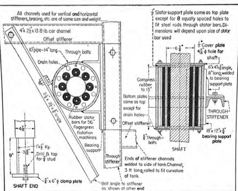
THE SUBMERGED BEARING, here seen in detail, supports the impeller shaft of agitator to prevent bending. See also page 55.
